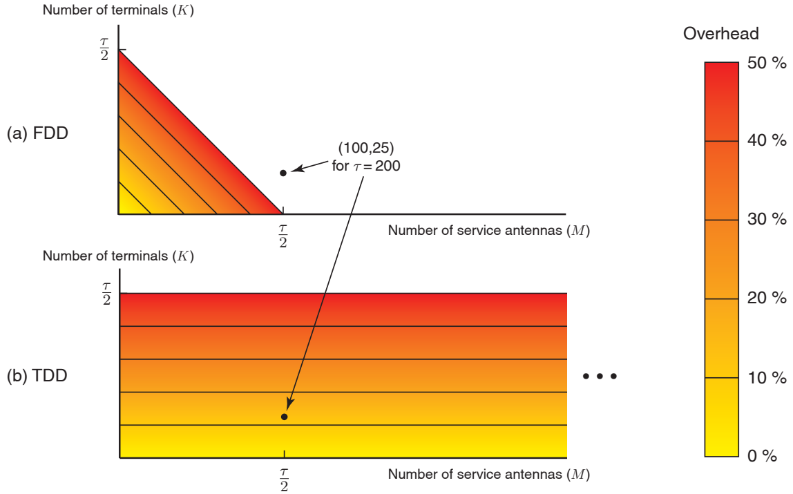
Fig. 6: Illustration of the typical overhead signaling in Massive MIMO based on (a) FDD and (b) TDD operation. The main difference is that FDD limits the number of antennas, while TDD can have any number of antennas. For a coherence block with \tau = 200 even a modest Massive MIMO setup with M = 100 and K = 25 is only supported in TDD operation.
