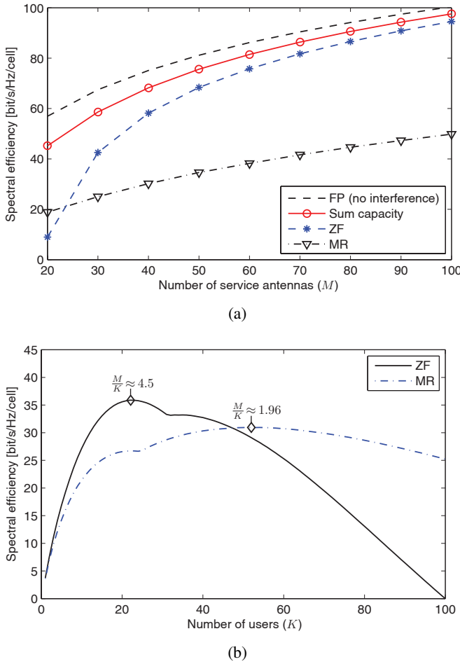
Fig. 4: Sum spectral efficiency for i.i.d. Rayleigh fading channels with linear processing. (a) The sum capacity achieved by DPC/SIC is compared with linear processing, assuming perfect CSI, no inter-cell interference, and K = 20 terminals. The loss incurred by linear processing is large when M \approx K , but reduces quickly as the number of antennas increases. In fact, ZF with around M + 10 antennas gives performance equivalent to the capacity with M antennas. (b) Performance in a multi-cellular system with a coherence block of \tau = 200 symbols, M = 100 service antennas, estimated CSI, and an SNR of -5 dB. The performance is shown as a function of K , with ZF and MR processing. The maximum at each curve is marked and it is clear that M/K < 10 at these operating points.
