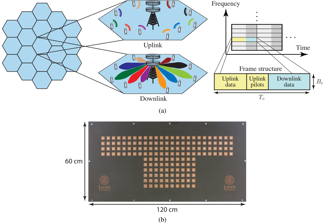
Fig. 1: Example of a Massive MIMO system. (a) Illustration of the uplink and downlink in line-of-sight propagation, where each BS is equipped with M antennas and serves K terminals. The TDD transmission frame consists of \tau = B_c T_c symbols. By capitalizing on channel reciprocity, there is payload data transmission in both the uplink and downlink, but only pilot transmission in the uplink. (b) Photo of the antenna array of the LuMaMi testbed at Lund University in Sweden [2]. The array consists of 160 dual-polarized patch antennas. It is designed for a carrier frequency of 3.7 GHz and the element-spacing is 4 cm (half a wavelength).
