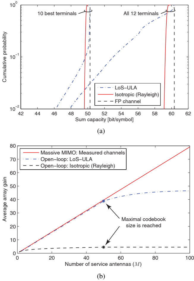
Fig. 2: Comparison of system behavior with i.i.d. Rayleigh fading respectively line-of-sight propagation. There are K = 12 terminals and \text{SNR}_u = -5 dB. (a) Cumulative distribution of the uplink sum capacity with M = 100 service antennas, when either all 12 terminals or only the 10 best terminals are served. (b) Average array gain achieved for different number of service antennas. The uplink channel estimation in Massive MIMO always provides a linear slope, while the performance of open-loop beamforming depends strongly on the propagation environment and codebook size.
