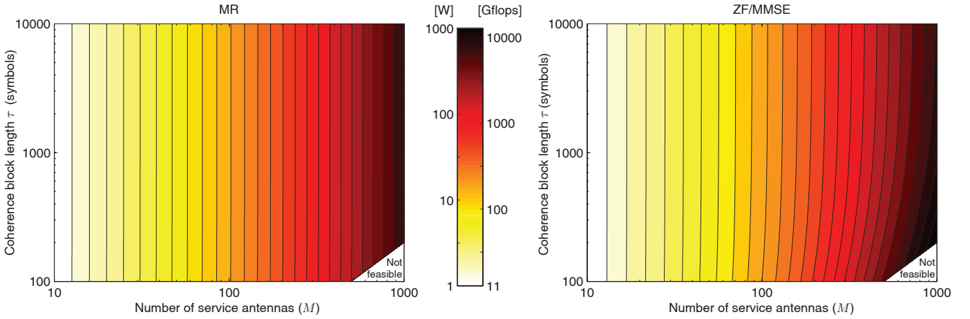
Fig. 5: Computational complexity (in flops) of the main baseband signal processing operations in an OFDM Massive MIMO setup: FFTs, channel estimation, precoding/combining of payload data, and computation of precoding/combining matrices. The complexity is also converted into an equivalent power consumption using a typical computational efficiency of 12.8 Gflops/Watt [15].
