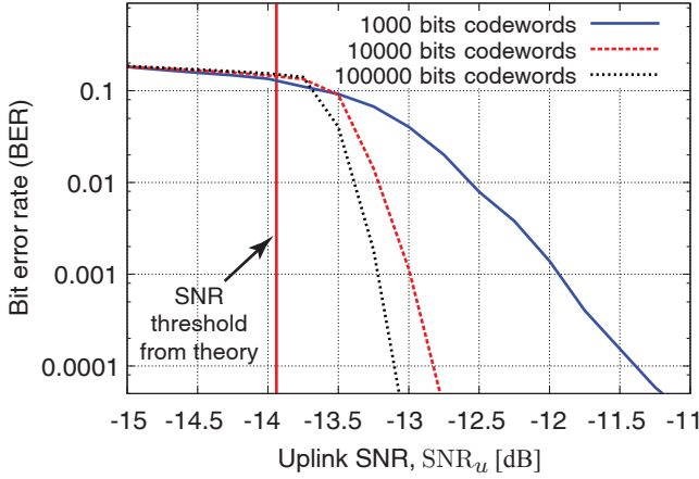
Fig. 3: Empirical uplink link performance of Massive MIMO with M = 100 antennas and K = 30 terminals using QPSK modulation with 1/2 coding rate and estimated channels. The vertical red line is the SNR threshold where zero BER can be achieved for infinitely long codewords, according to the spectral efficiency expression in Eq. (1).
